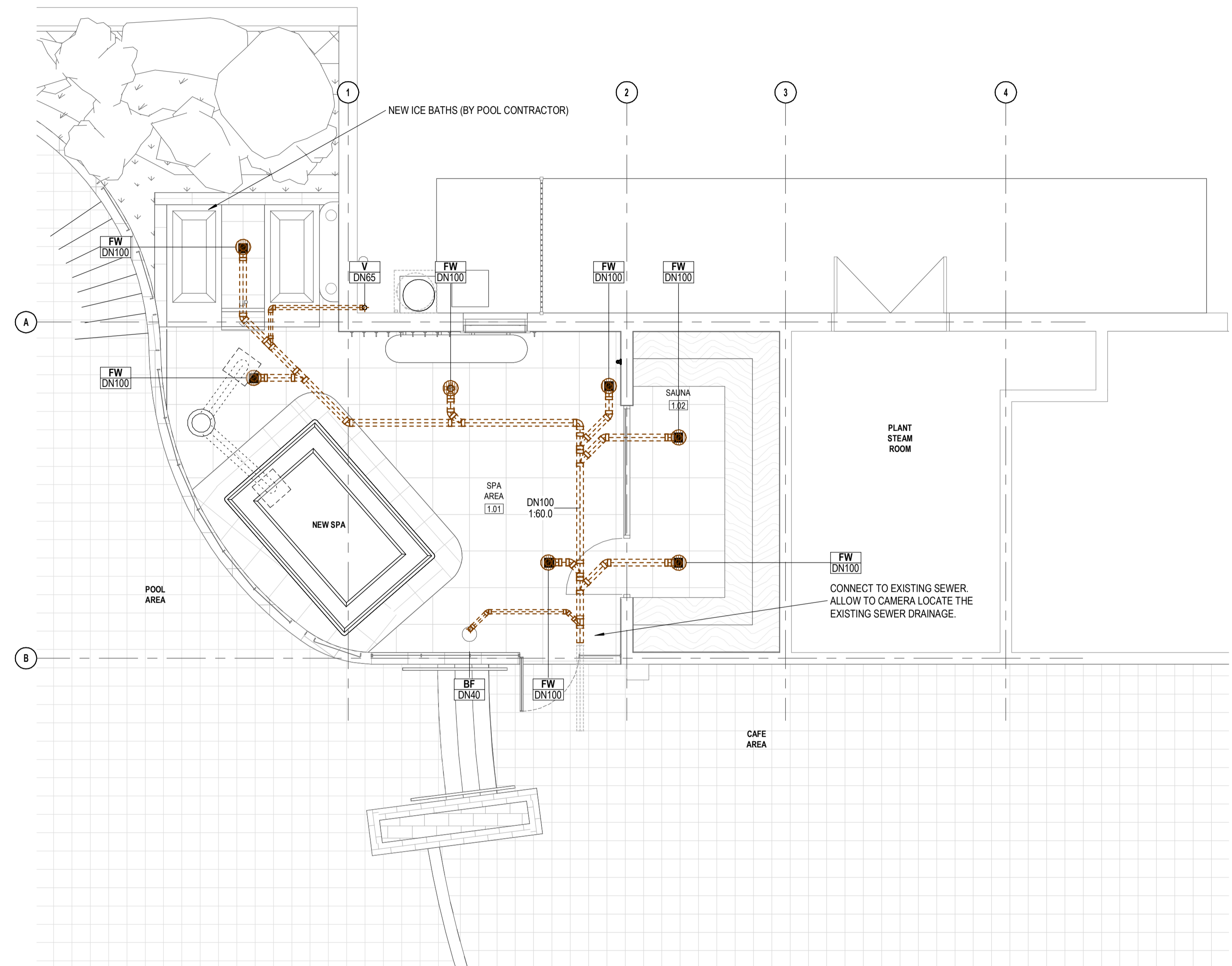
SPA FLOOR - SEWER LAYOUT 1:50
