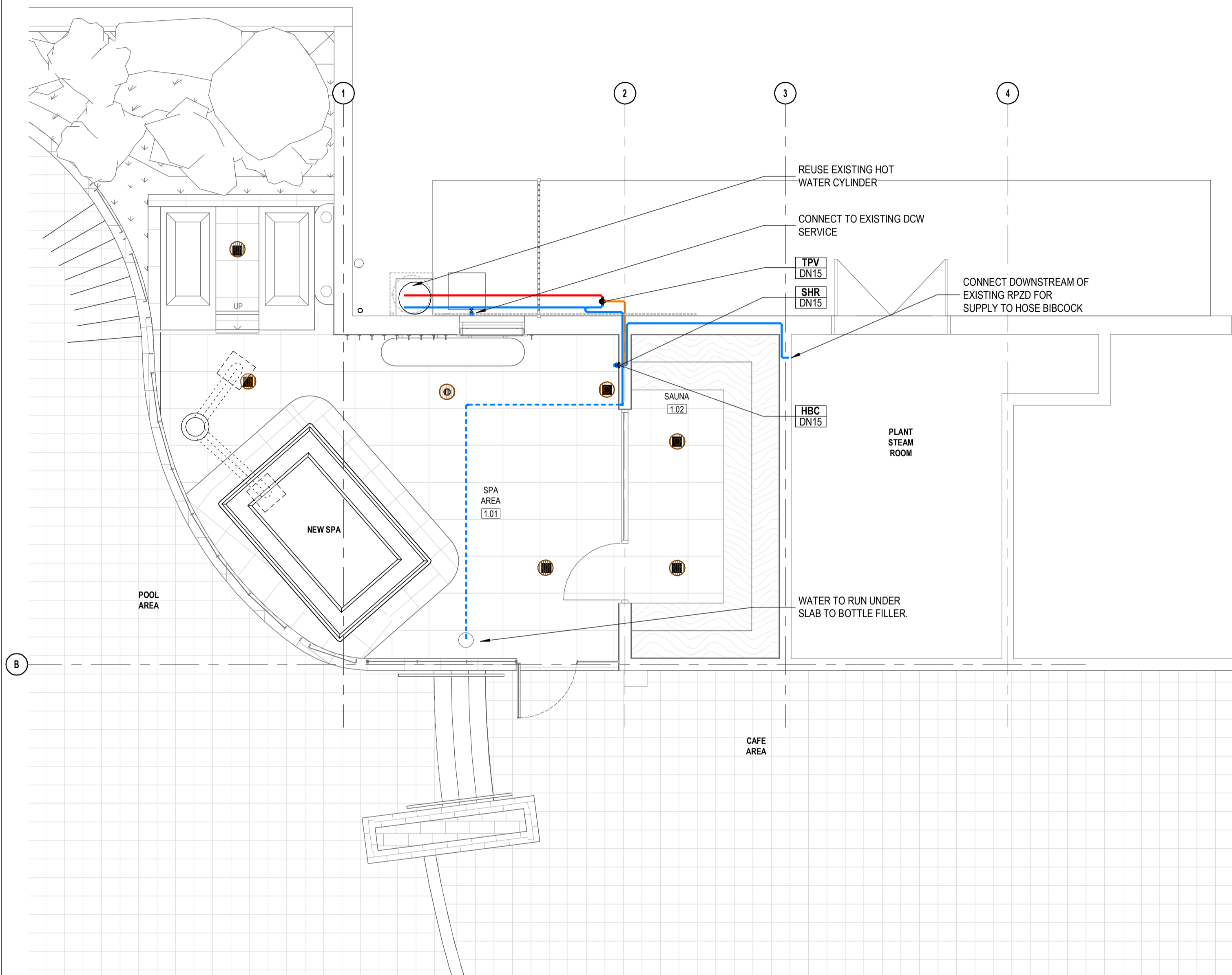
SPA FLOOR - WATER RETICULATION LAYOUT 1:50
